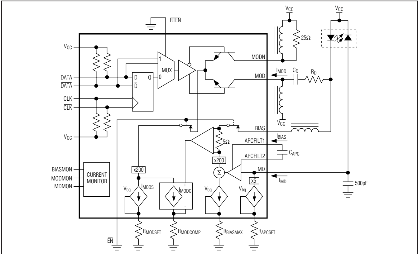
Figure 3. Functional Diagram
