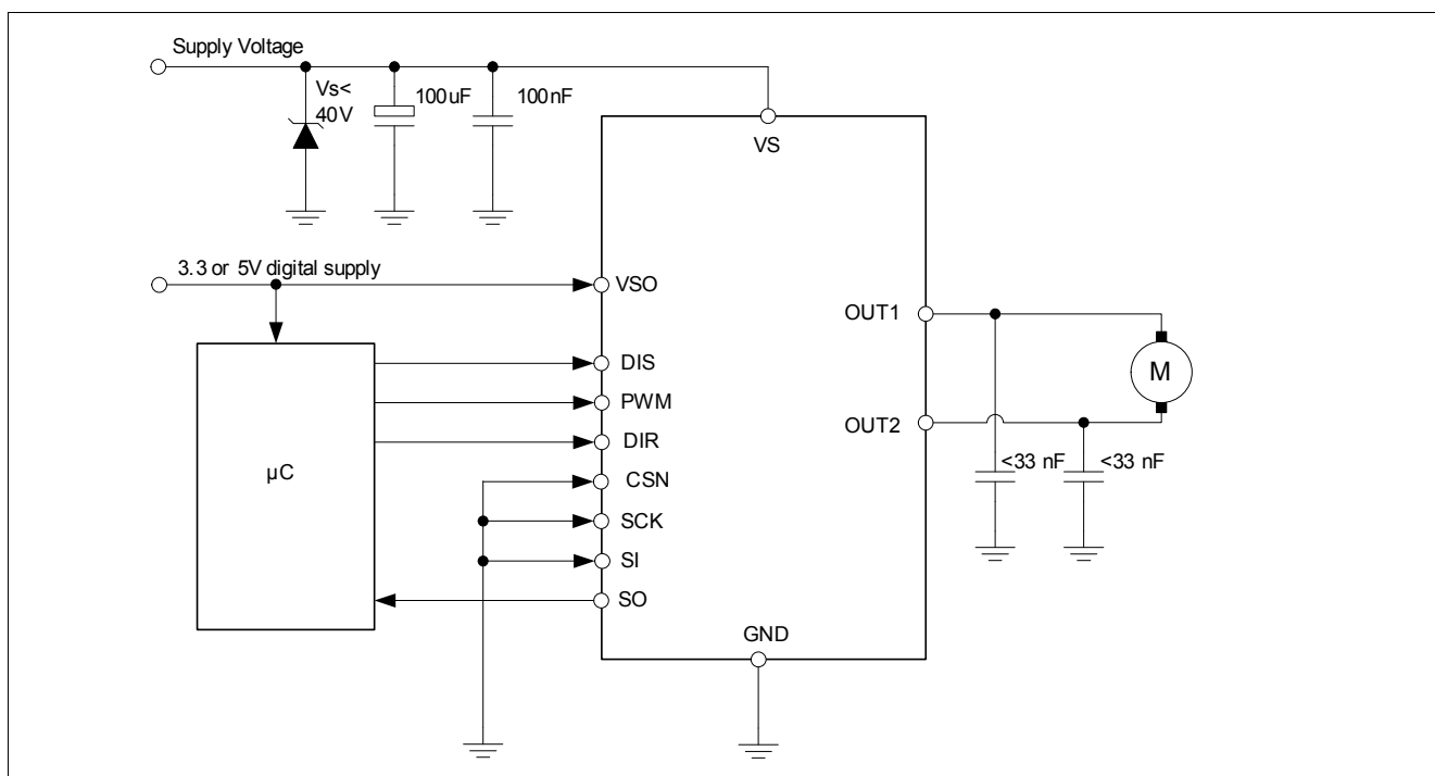
Figure 5 Application Example H-Bridge with Error Flag
