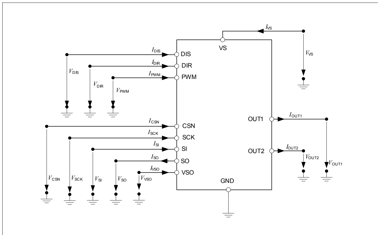
Figure 2 Terms IFX9201SG
