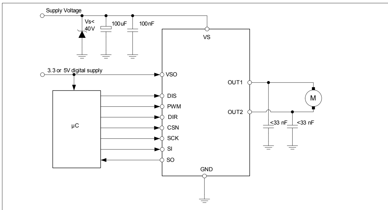
Figure 4 Application Example H-Bridge with SPI interface
