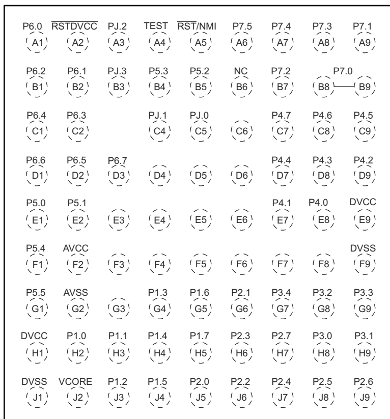
Figure 7-5. 80-Pin ZHX or ZQE Package (Top View) – MSP430F5249, MSP430F5247, MSP430F5239, MSP430F5237
