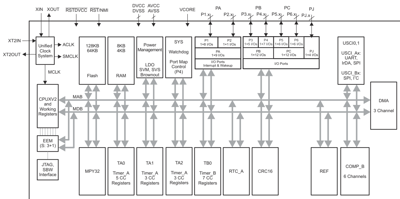
Figure 4-4. Functional Block Diagram – F5234, F5232 – RGZ Package
