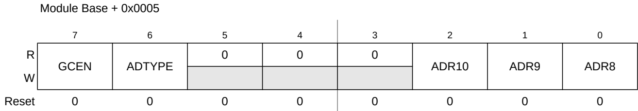
Figure 10-9. IIC Bus Control Register 2(BCR2)
