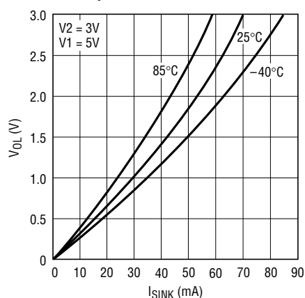
RST, COMPX Voltage Output Low vs Output Sink Current
