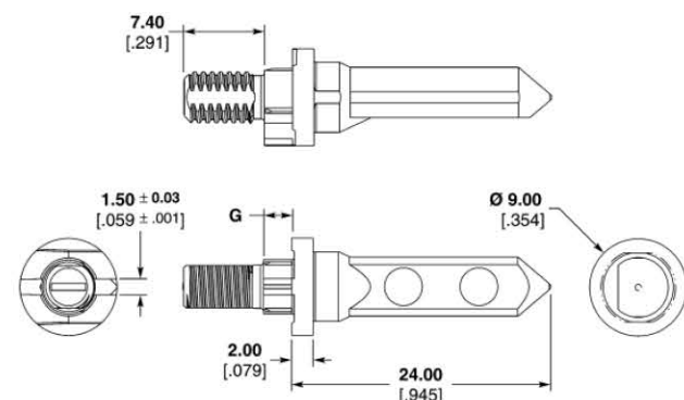
Pin Part Number 1-1469491-X
