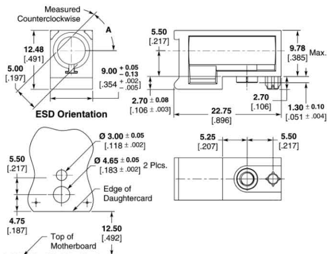
Guide Module Part Number 1-1469492-X
