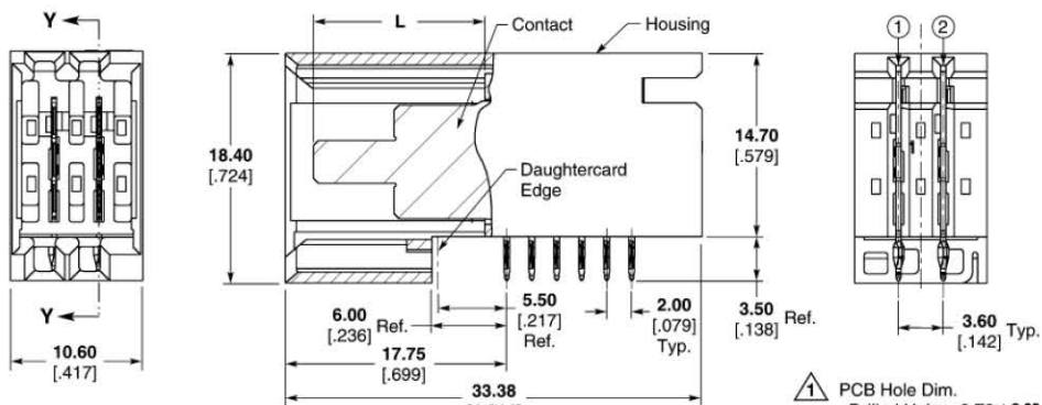
Section Y-Y
