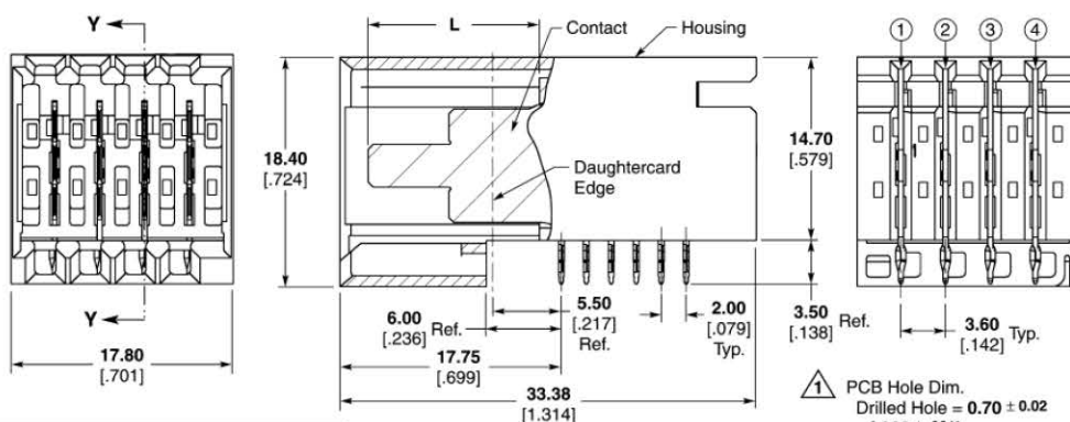
Section Y-Y
