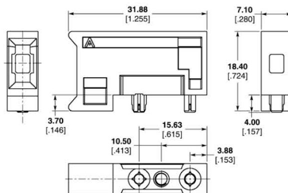
Guide Module Part Number 1410714-2
