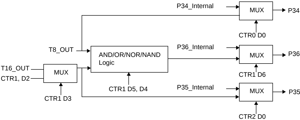
Figure 26. Output Circuit
