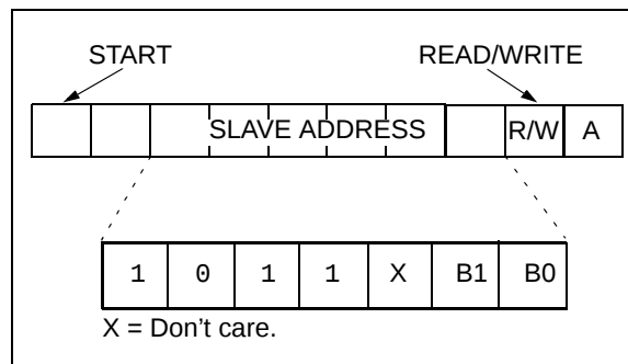
FIGURE 4-2: CONTROL BYTE ALLOCATION
