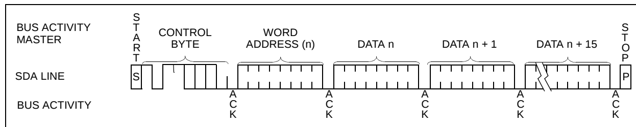
FIGURE 5-2: PAGE WRITE
