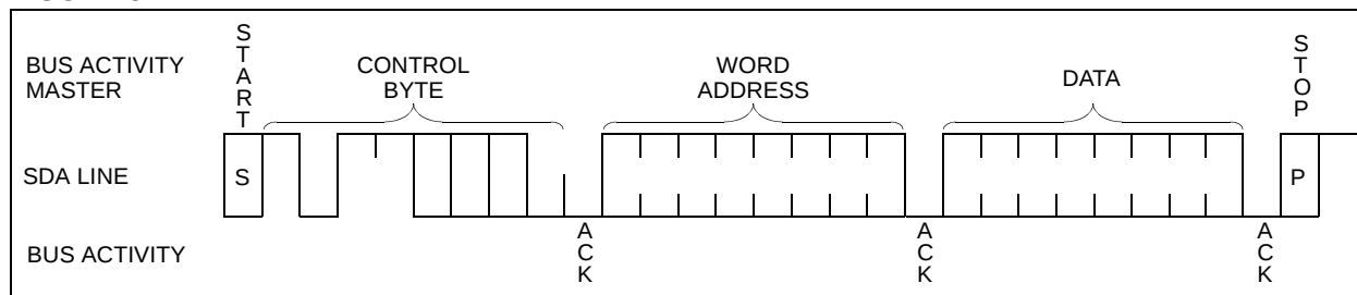
FIGURE 5-1: BYTE WRITE
