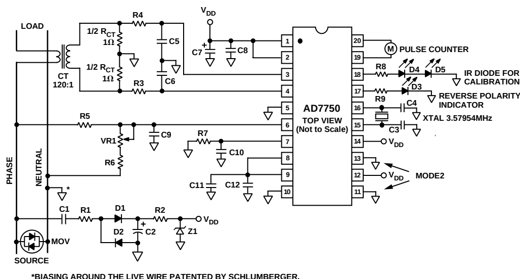
Figure 21. Suggested Class 1 Meter Implementation
