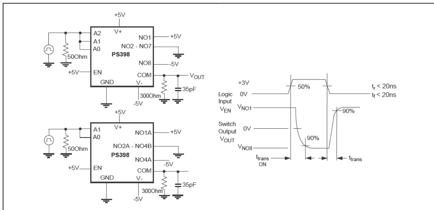
Figure 1. Transition Time
