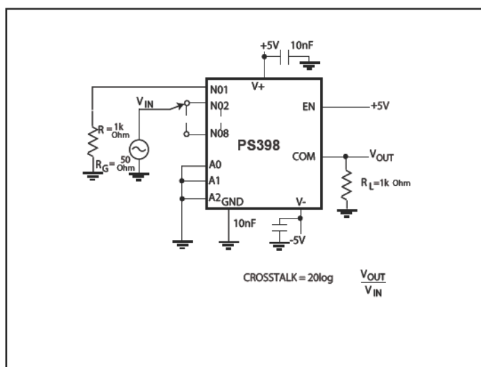
Figure 6. CrossTalk
