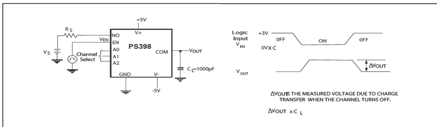
Figure 4. Charge Injection
