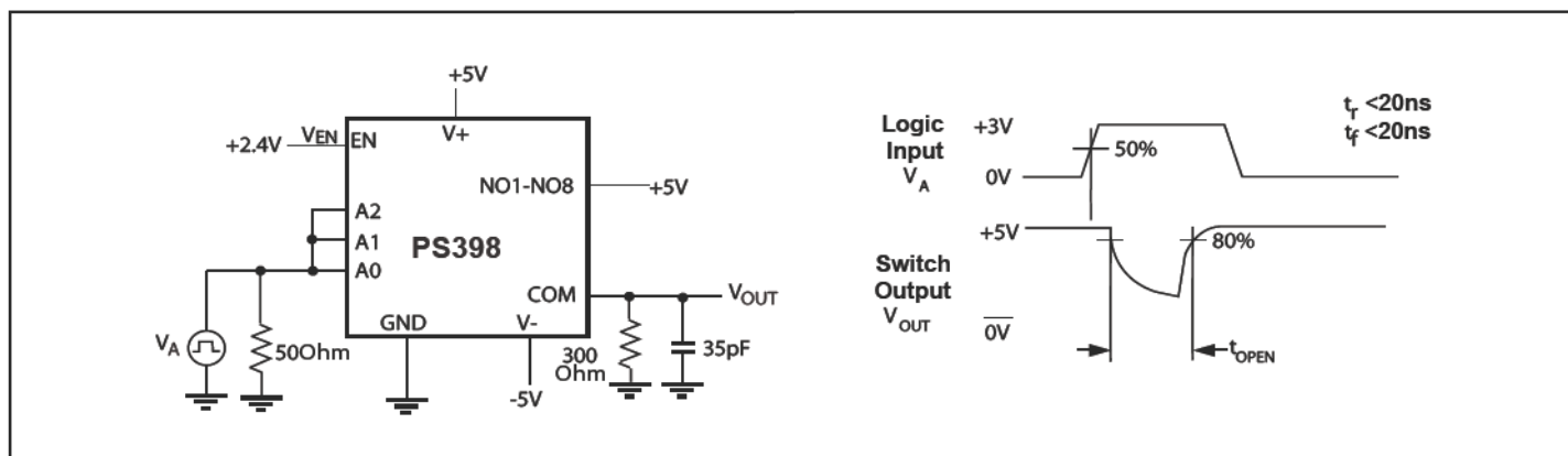
Figure 3. Break-Before-Make Interval
