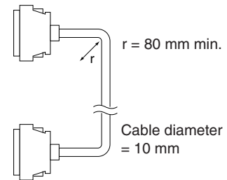
CV-series Long-distance I/O Connecting Cable
