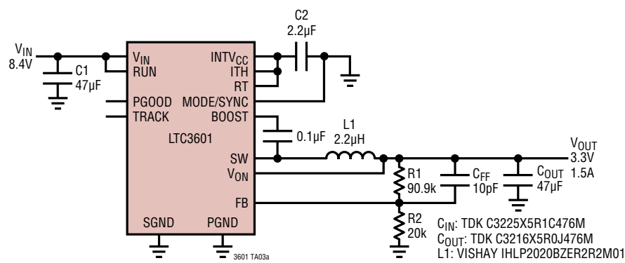
8.4V Input to 3.3V Output at 2MHz Operating Frequency Using Forced Continuous Mode
