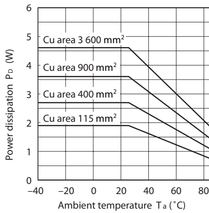
Fig.20 Power Dissipation vs. Ambient Temperature (Typical Value)
