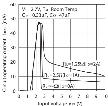
Fig.15 Circuit Operating Current vs. Input Voltage (PQ025EH02ZxH)
