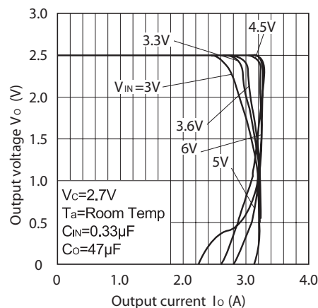
Fig.6 Overcurrent Protection Characteristics (PQ025EH02ZxH)
