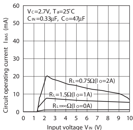
Fig.13 Circuit Operating Current vs. Input Voltage (PQ015EH02ZxH)
