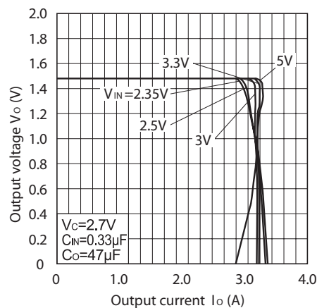
Fig.4 Overcurrent Protection Characteristics (PQ015EH02ZxH)
