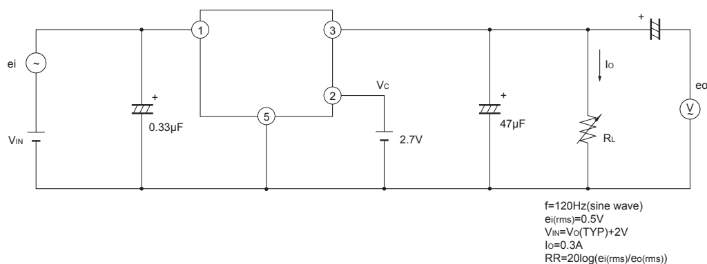
Fig.2 Test circuit of Ripple Rejection
