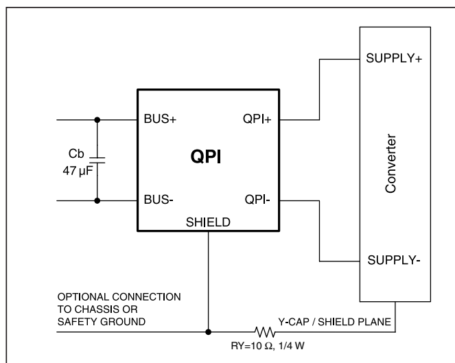
Figure 1 - QPI-3 circuit on input bus.
