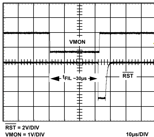
FIGURE 5. \overline{VMON} LOW TO \overline{RST} LOW
