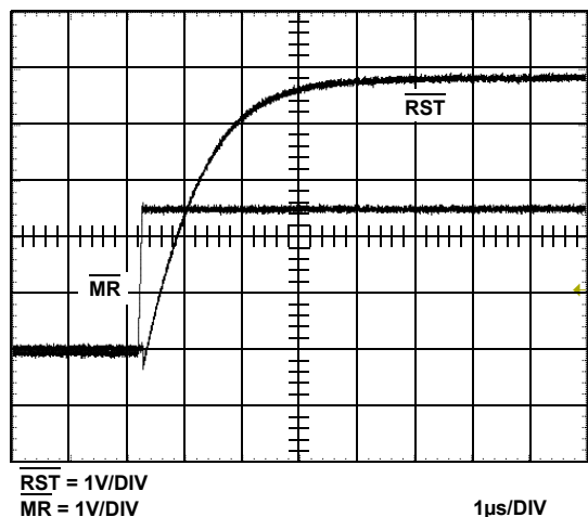
FIGURE 6. \overline{MR} HIGH TO \overline{RST} HIGH
