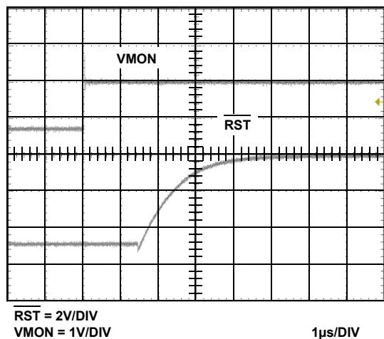
FIGURE 4. \overline{VMON} HIGH TO \overline{RST} HIGH
