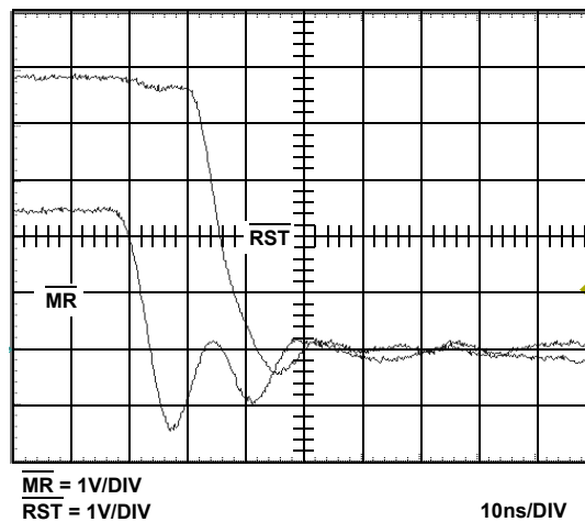
FIGURE 7. \overline{MR} LOW TO \overline{RST} LOW
