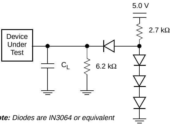
Figure 8. Test Setup
