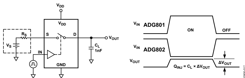
Figure 17. Charge Injection
