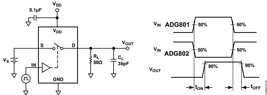
Figure 16. Switching Times
