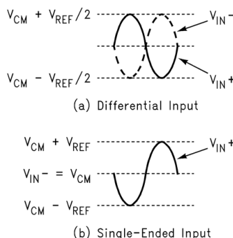
Figure 31. Expected Input Signal Range
