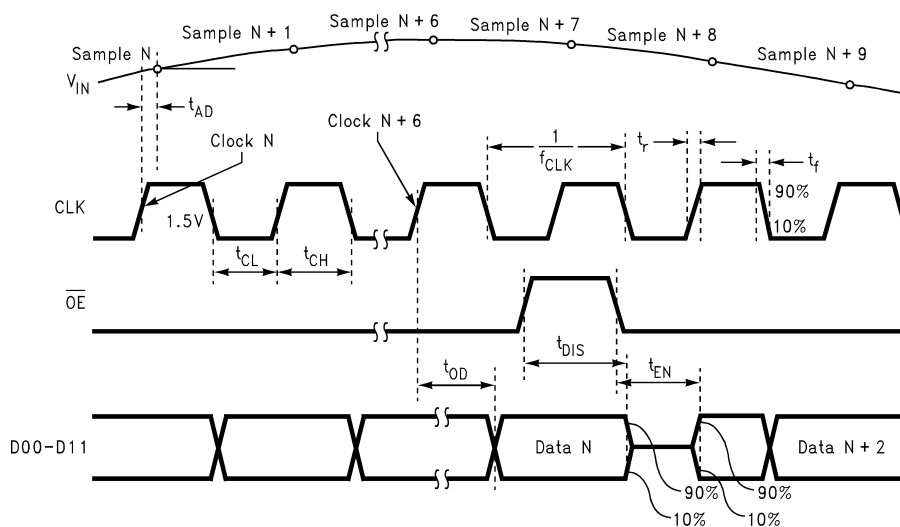
Figure 3. Output Timing
