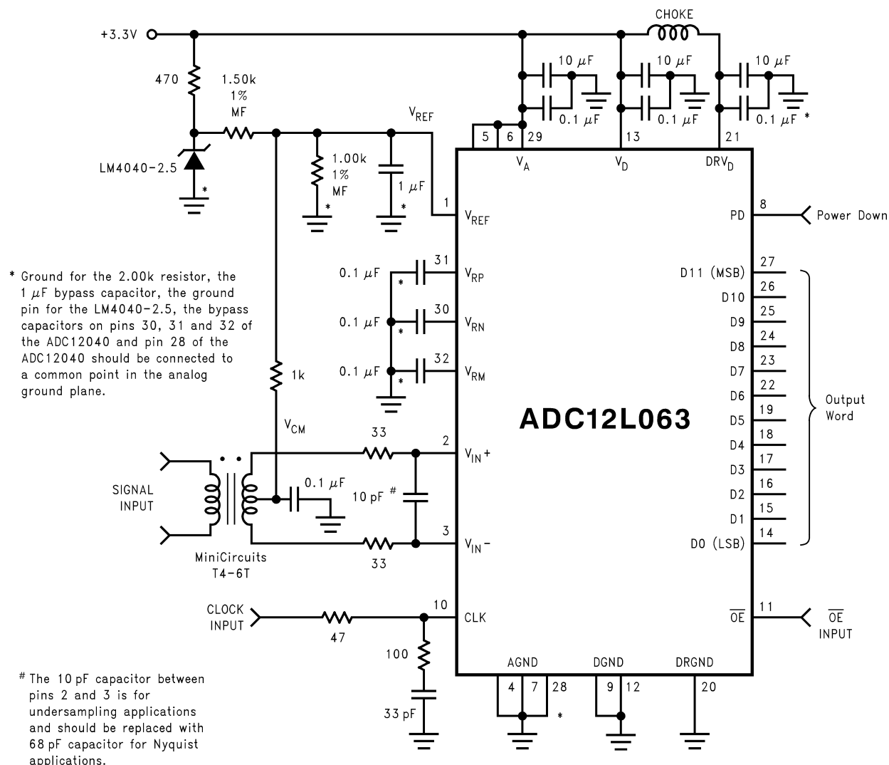
Figure 35. Driving the Signal Inputs with a Transform
