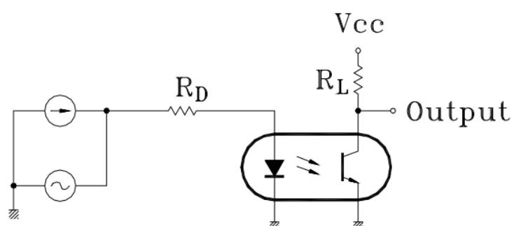
Frequency Response Test Circuit
