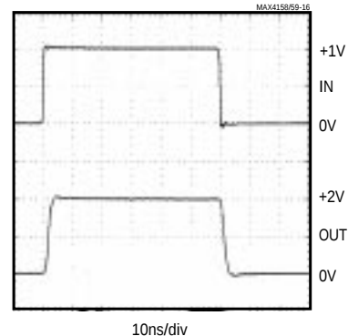
MAX4258/MAX4259 LARGE-SIGNAL PULSE RESPONSE
