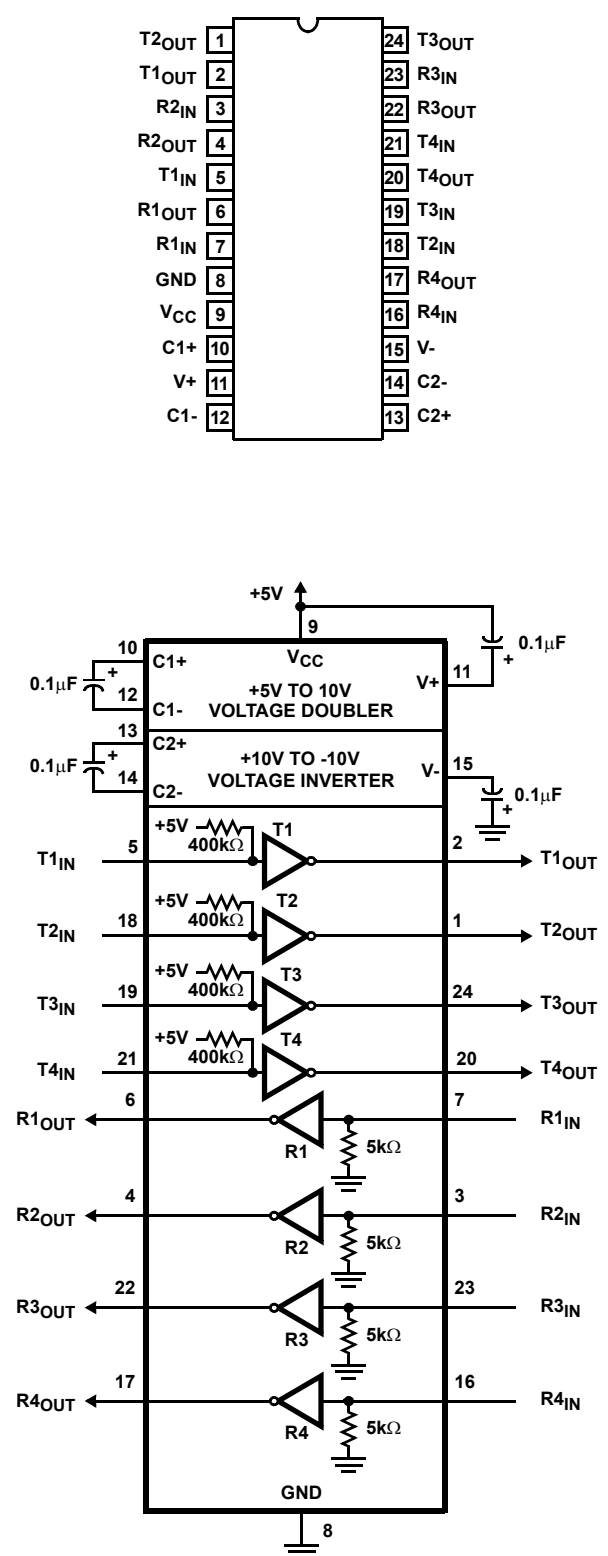
HIN208 (SOIC) TOP VIEW
