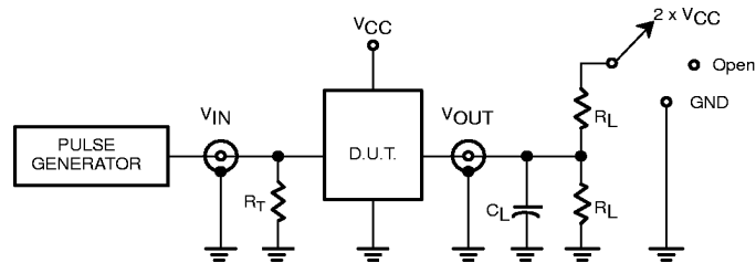
Test Circuit for 3-State Outputs
