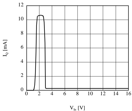
■ I_{\text{Q}} vs V_{\text{In}} (AP1155ADL)
