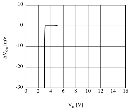
■ \Delta V_{\text{Out}} vs V_{\text{In}} (AP1155ADL)
