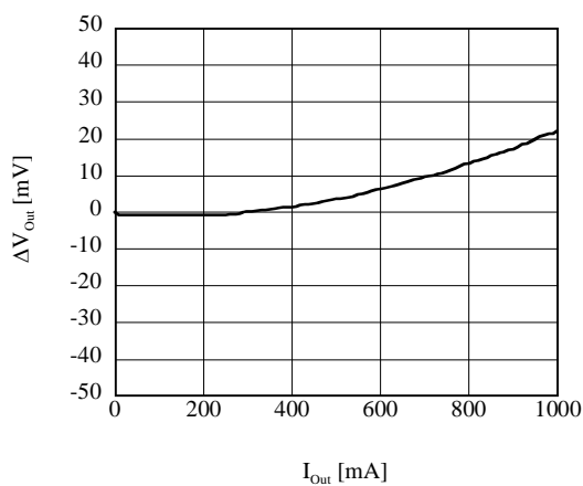
■ \Delta V_{\text{Out}} vs I_{\text{Out}} (AP1155ADL)
