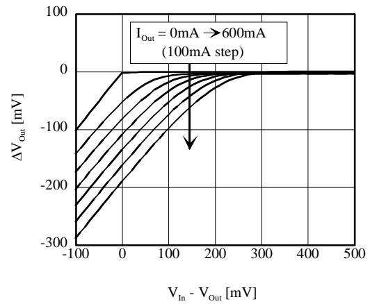
■ \Delta V_{\text{Out}} vs V_{\text{In}} (AP1155ADL)
