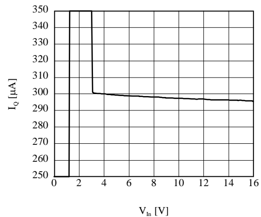
■ I_{\text{Q}} vs V_{\text{In}} (AP1155ADL)
