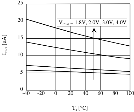
■ I_{\text{Cont}} vs T_a (AP1155ADL)
