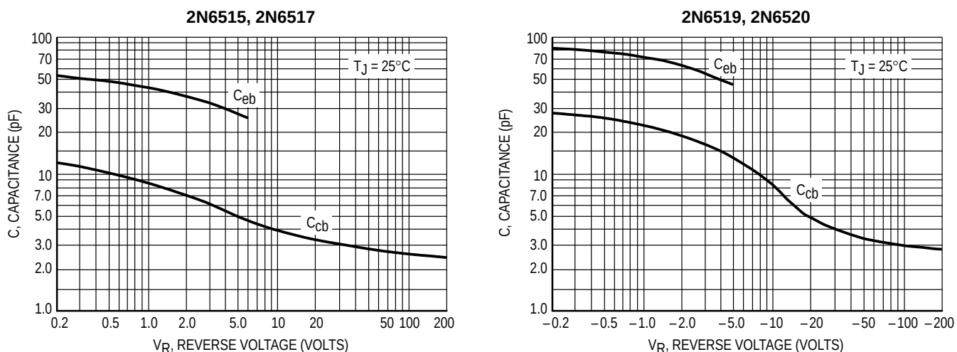
Figure 6. Capacitance
