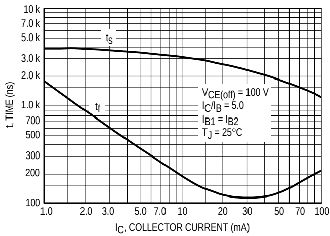
Figure 8. Turn-Off Time
