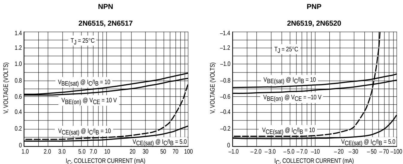
Figure 4. "On" Voltages
