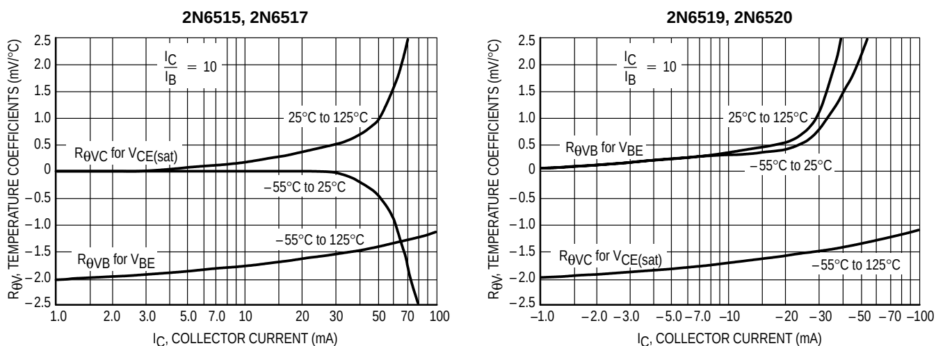
Figure 5. Temperature Coefficients
