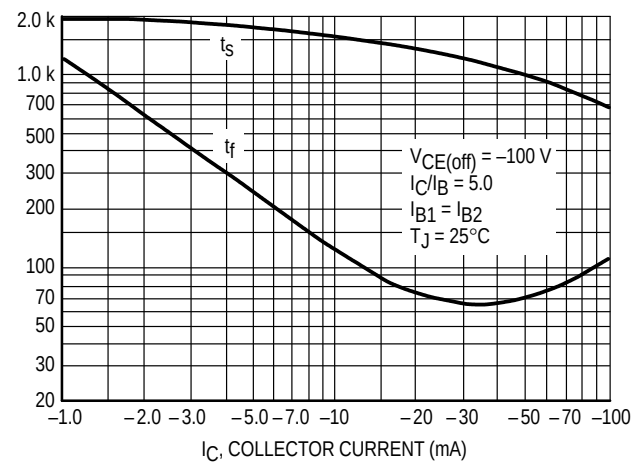
Figure 8. Turn-Off Time
