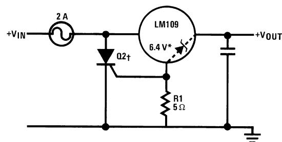
Figure 3. Input Crowbar
