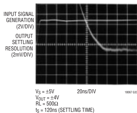
0.01% Settling Time
