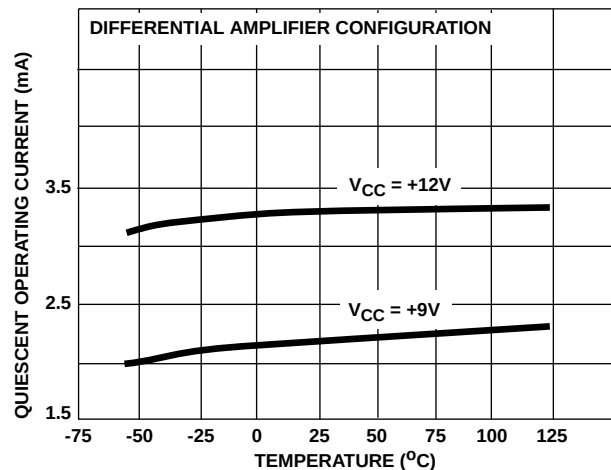
FIGURE 18. QUIESCENT OPERATING CURRENT vs TEMPERATURE FOR CA3053
