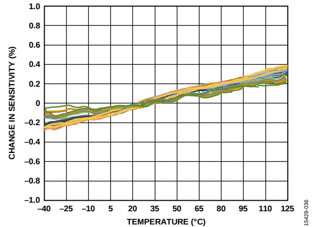
Figure 36. ADXL357 Y-Axis Change in Sensitivity Relative to 25°C vs. Temperature
