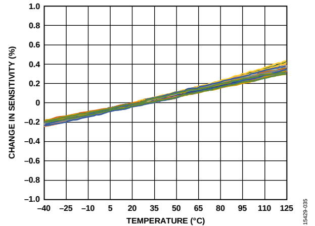
Figure 35. ADXL357 X-Axis Change in Sensitivity Relative to 25°C vs. Temperature
