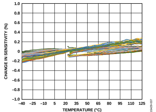
Figure 37. ADXL357 Z-Axis Change in Sensitivity Relative to 25°C vs. Temperature
