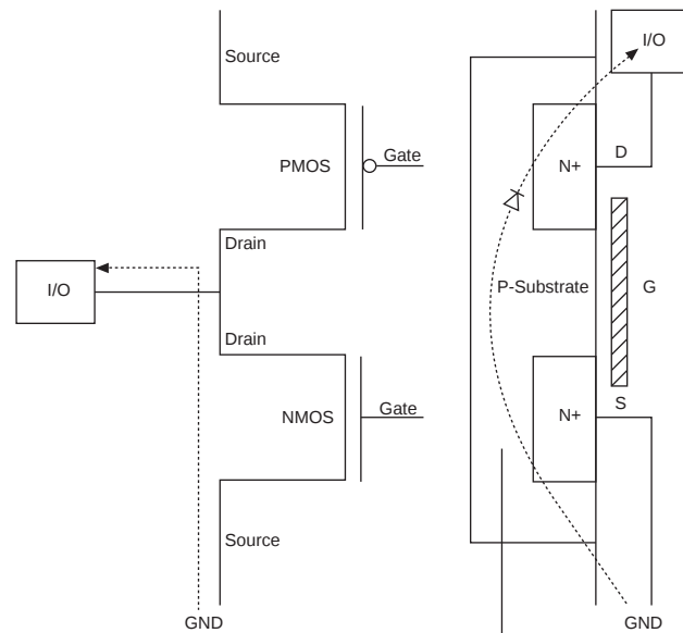
Figure 4-4. ESD Protection During Negative Voltage Zap
