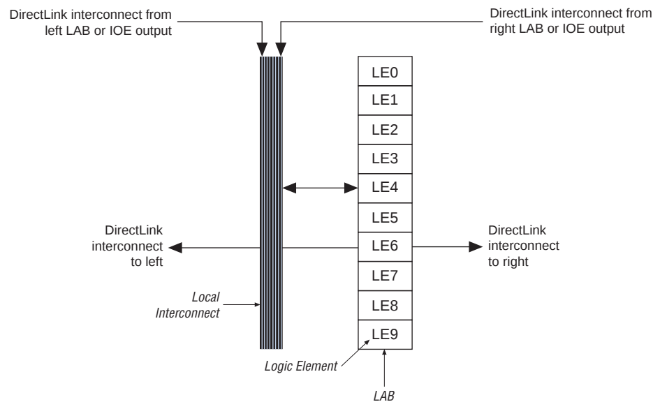
Figure 2-4. DirectLink Connection
