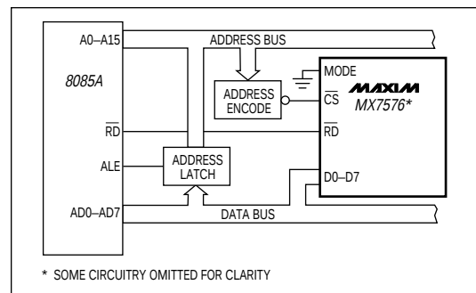
Figure 10. MX7575 to 8085A Asynchronous Conversion Mode Interface
