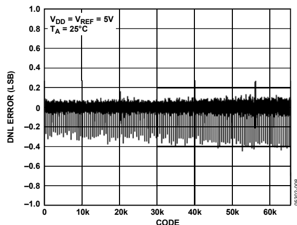
Figure 8. DNL AD5668—External Reference
