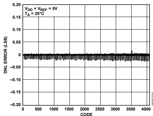
Figure 10. DNL AD5628—External Reference
