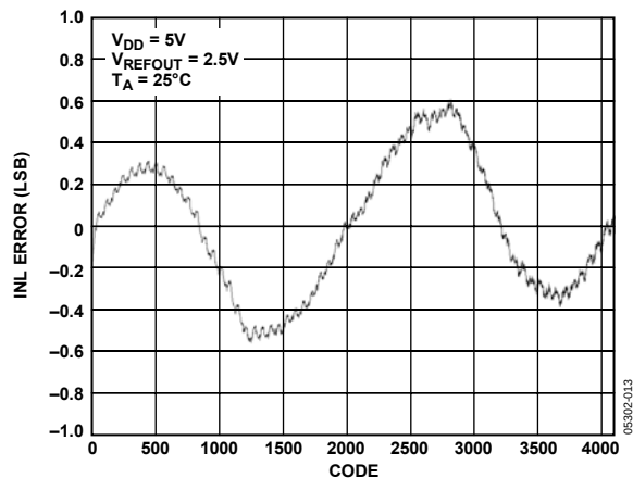
Figure 13. INL AD5628-2
