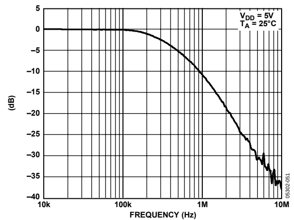
Figure 50. Multiplying Bandwidth
