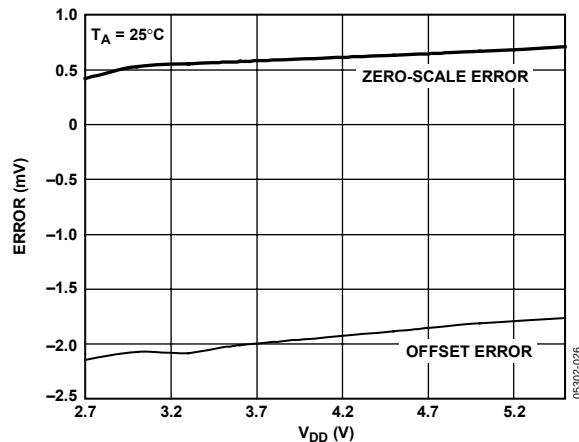
Figure 26. Zero-Scale Error and Offset Error vs. Supply Voltage
