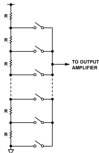
Figure 52. Resistor String
