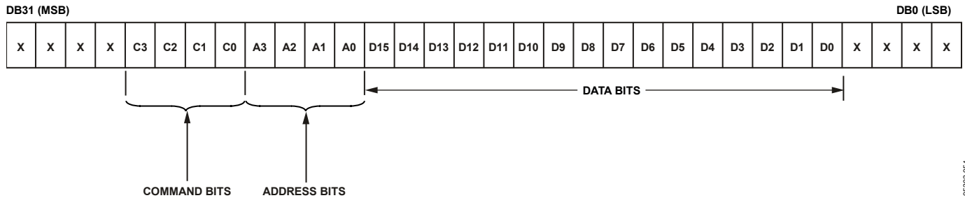
Figure 53. AD5668 Input Register Contents
