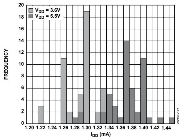
Figure 27. I_{DD} Histogram with External Reference
