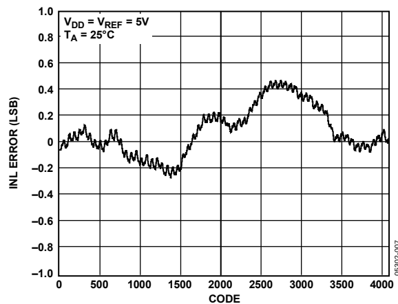
Figure 7. INL AD5628—External Reference
