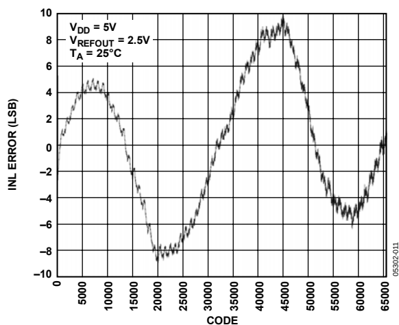
Figure 11. INL AD5668-2/AD5668-3
