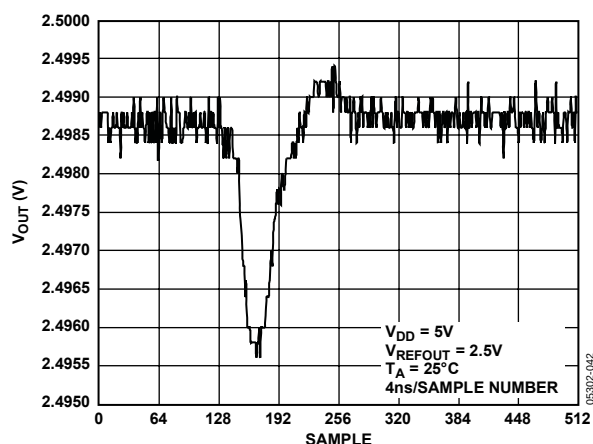
Figure 41. Analog Crosstalk
