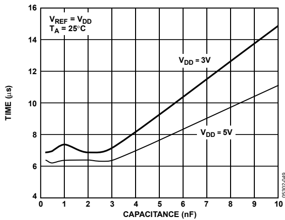
Figure 48. Settling Time vs. Capacitive Load
