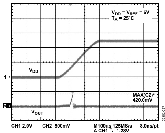
Figure 37. Power-On Reset to 0 V
