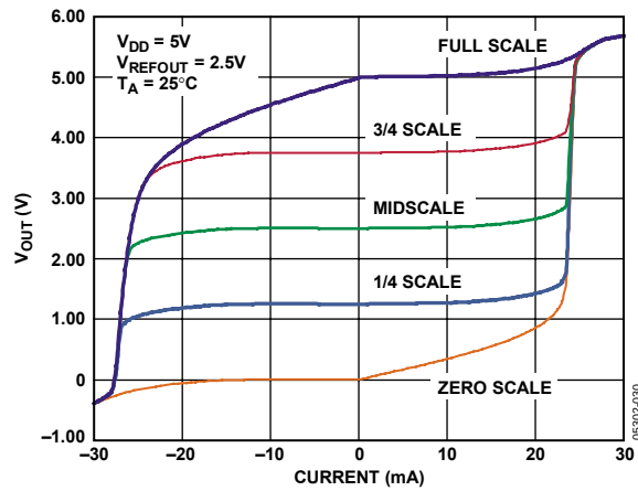
Figure 30. AD5668-2/AD5668-3 Source and Sink Capability
