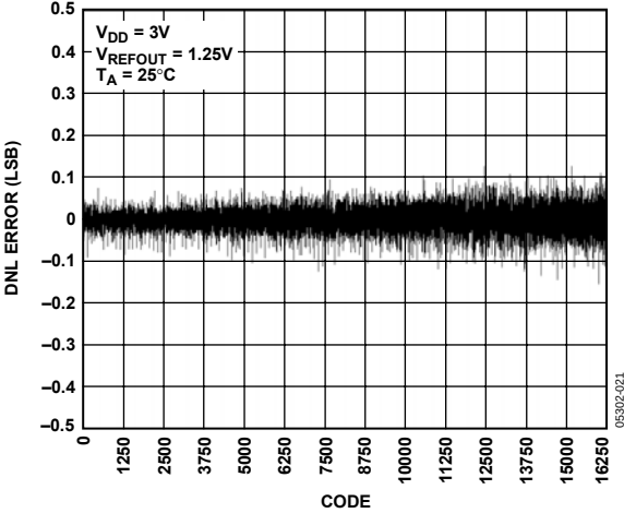
Figure 21. DNL AD5648-1
