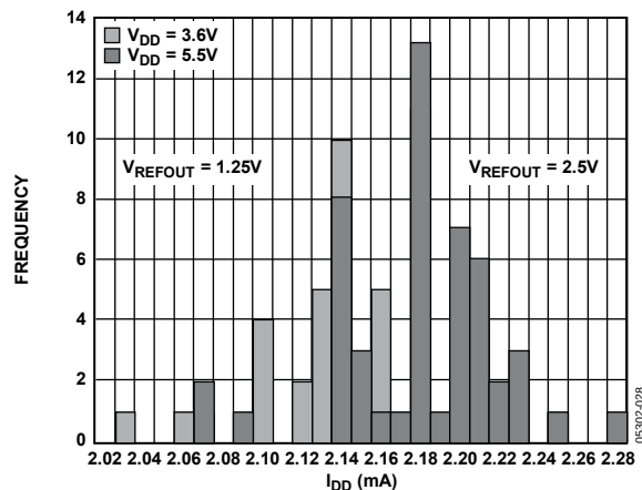
Figure 28. I_{DD} Histogram with Internal Reference
