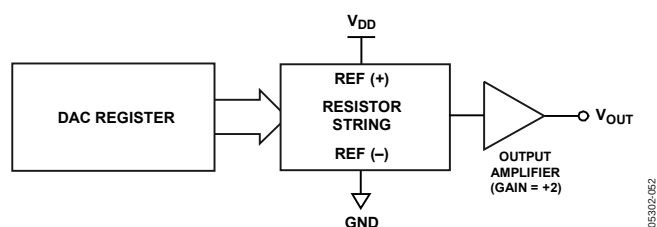
Figure 51. DAC Architecture
