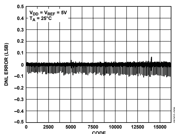
Figure 9. DNL AD5648—External Reference
