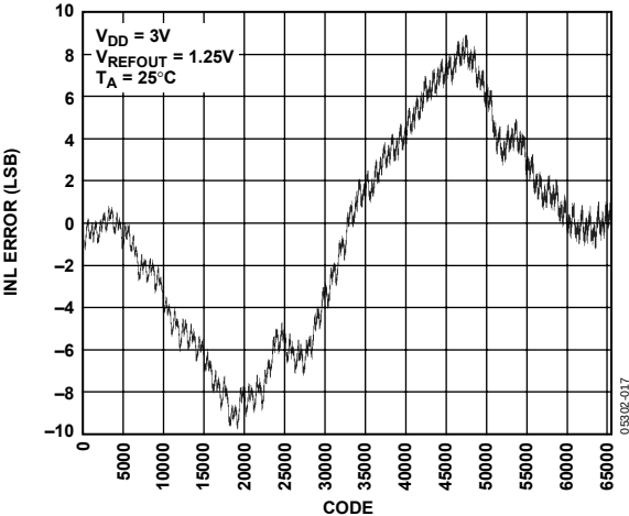
Figure 17. INL AD5668-1
