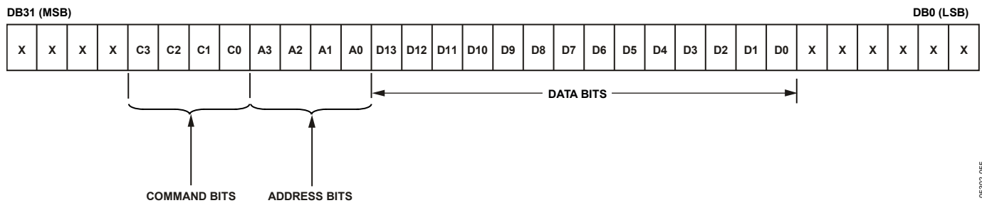
Figure 54. AD5648 Input Register Contents
