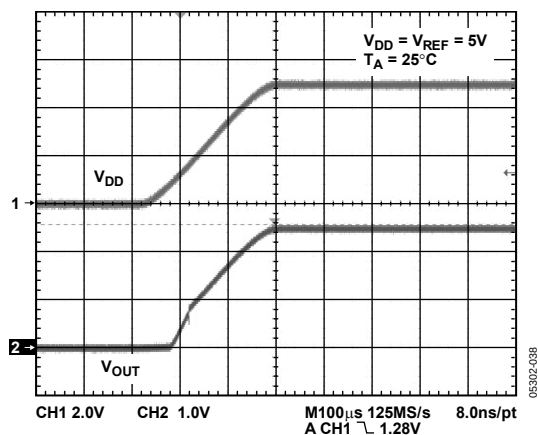
Figure 38. Power-On Reset to Midscale
