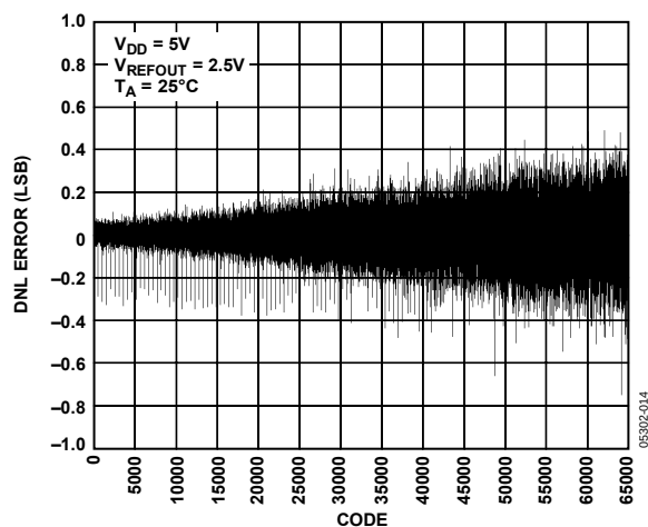
Figure 14. DNL AD5668-2/AD5668-3
