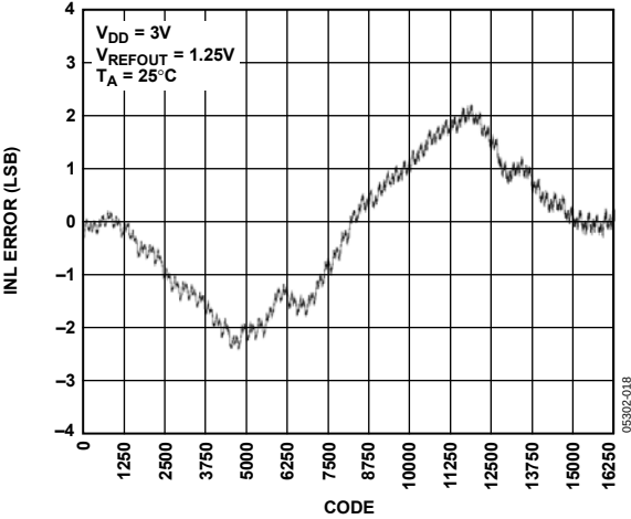
Figure 18. INL AD5648-1
