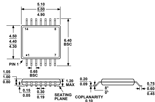
Figure 58. 14-Lead Thin Shrink Small Outline Package [TSSOP] (RU-14)
