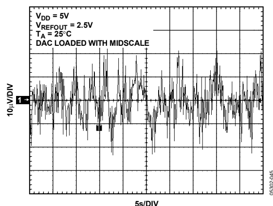
Figure 44. 0.1 Hz to 10 Hz Output Noise Plot, Internal Reference
