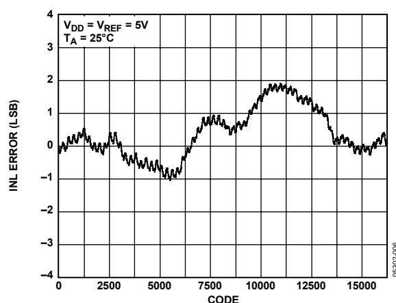
Figure 6. INL AD5648—External Reference
