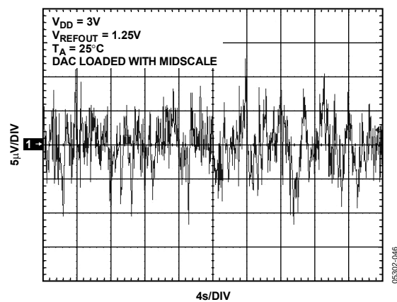
Figure 45. 0.1 Hz to 10 Hz Output Noise Plot, Internal Reference
