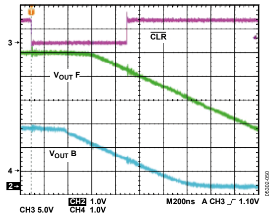
Figure 49. Hardware \overline{CLR}
