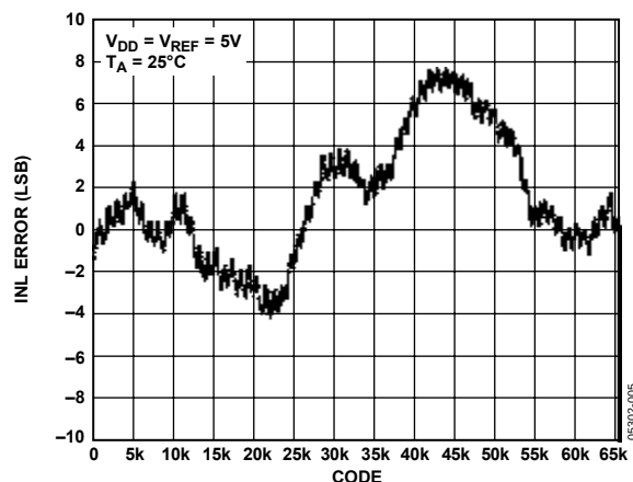
Figure 5. INL AD5668—External Reference
