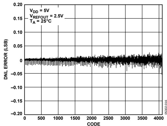
Figure 16. DNL AD5628-2
