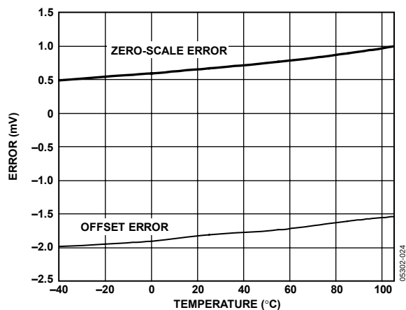
Figure 24. Zero-Scale Error and Offset Error vs. Temperature
