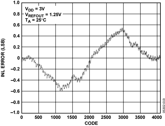
Figure 19. INL AD5628-1
