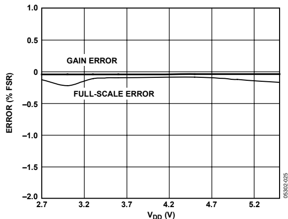
Figure 25. Gain Error and Full-Scale Error vs. Supply Voltage
