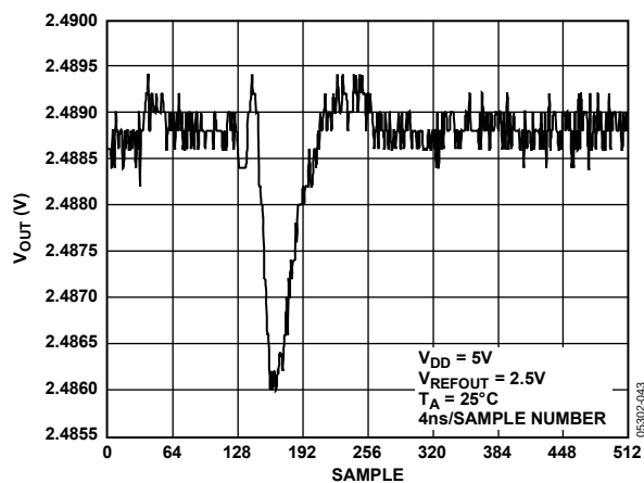
Figure 42. DAC-to-DAC Crosstalk
