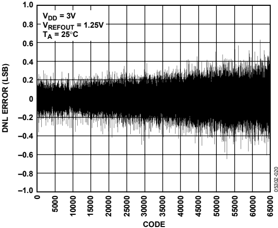
Figure 20. DNL AD5668-1
