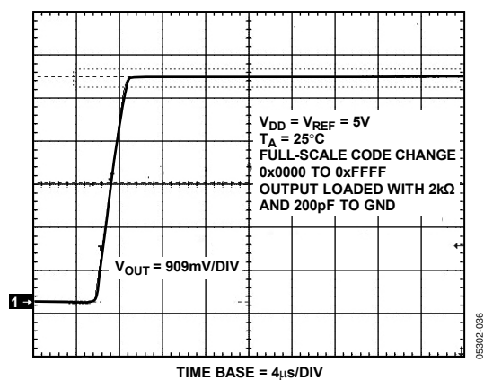
Figure 36. Full-Scale Settling Time, 5 V
