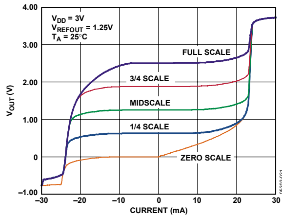
Figure 31. AD5668-1 Source and Sink Capability
