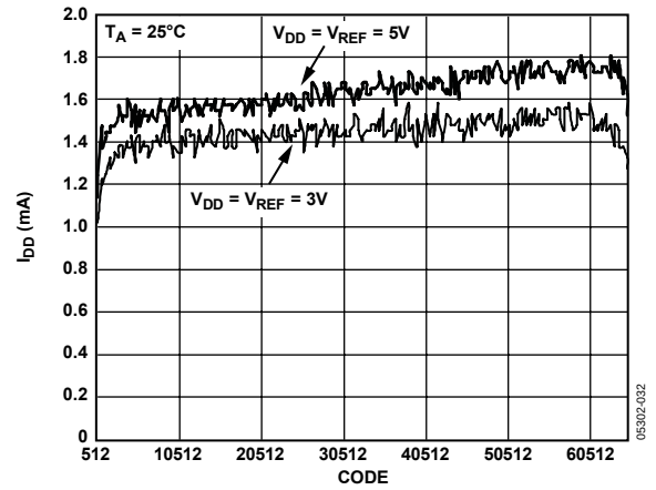
Figure 32. Supply Current vs. Code
