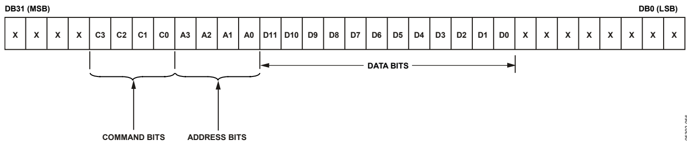
Figure 55. AD5628 Input Register Contents
