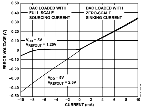
Figure 29. Headroom at Rails vs. Source and Sink
