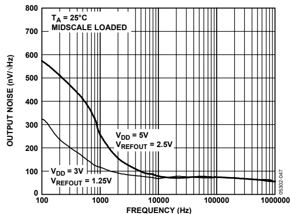
Figure 46. Noise Spectral Density, Internal Reference
