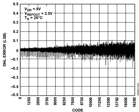
Figure 15. DNL AD5648-2
