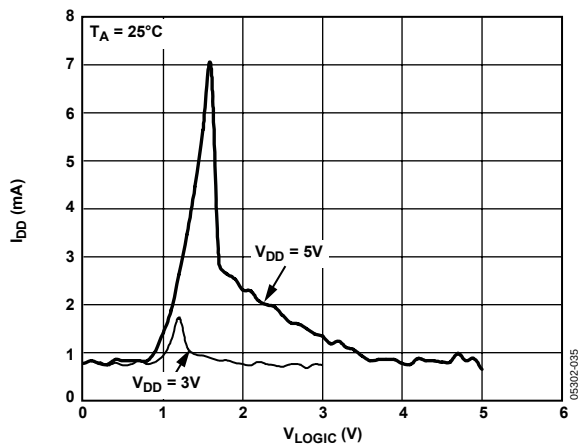
Figure 35. Supply Current vs. Logic Input Voltage
