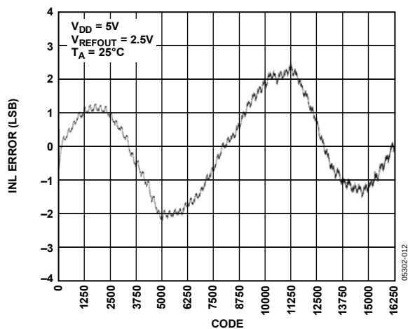
Figure 12. INL AD5648-2
