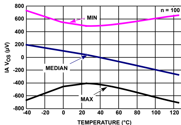
FIGURE 46. IA INPUT OFFSET VOLTAGE vs TEMPERATURE V_+, V_- = \pm 1.2V
