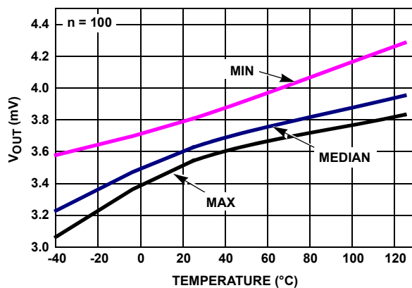
FIGURE 60. V_{OUT} LOW vs TEMPERATURE R_L = 100k , V_+, V_- = \pm 2.5V
