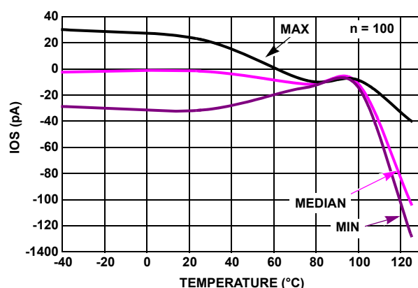
FIGURE 44. INPUT OFFSET CURRENT vs TEMPERATURE, V_+, V_- = \pm 1.2V
