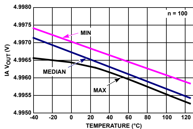
FIGURE 54. IA V_{OUT} HIGH vs TEMPERATURE, R_L = 100k , V_+ = +2.5V , V_- = -2.5V
