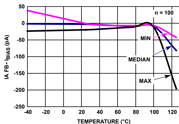
FIGURE 32. I_{BIAS} (IA FB-) vs TEMPERATURE, V_+ , V_- = \pm 1.2V
