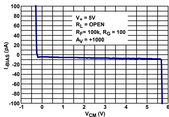
FIGURE 14. INPUT BIAS CURRENT vs COMMON-MODE INPUT VOLTAGE
