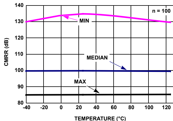
FIGURE 50. CMRR vs TEMPERATURE, V_{CM} = +2.5V TO -2.5V
