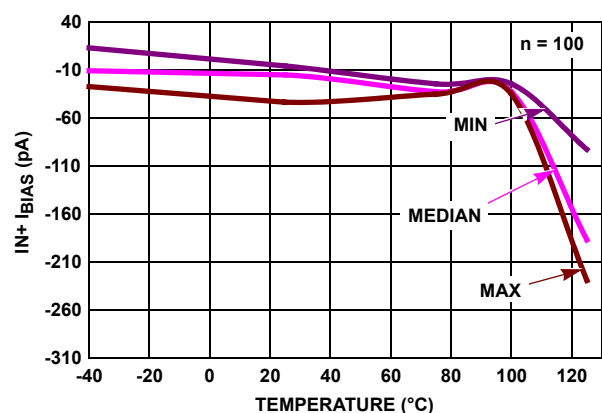
FIGURE 39. I_{BIAS} (IN+) vs TEMPERATURE, V_+ , V_- = \pm 1.2V
