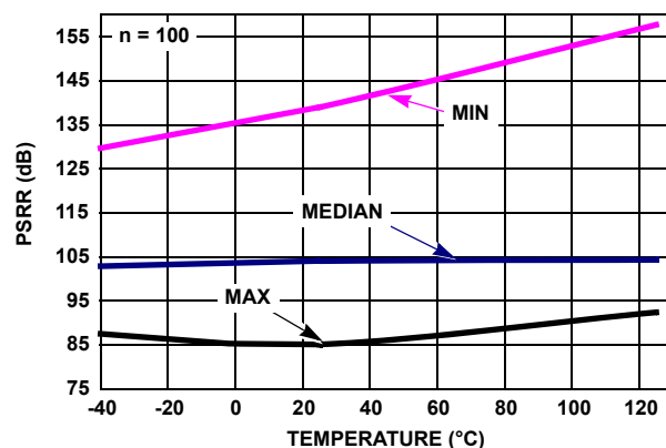
FIGURE 52. PSRR vs TEMPERATURE, V_+ = +2.5V , V_- = -2.5V
