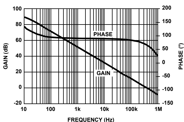
FIGURE 16. AMPLIFIER "B" (OP AMP) A_{VOL} vs FREQUENCY @ 1k \Omega LOAD
