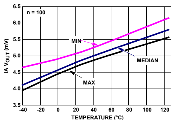
FIGURE 56. IA V_{OUT} LOW vs TEMPERATURE, R_L = 100k , V_+, V_- = \pm 2.5V
