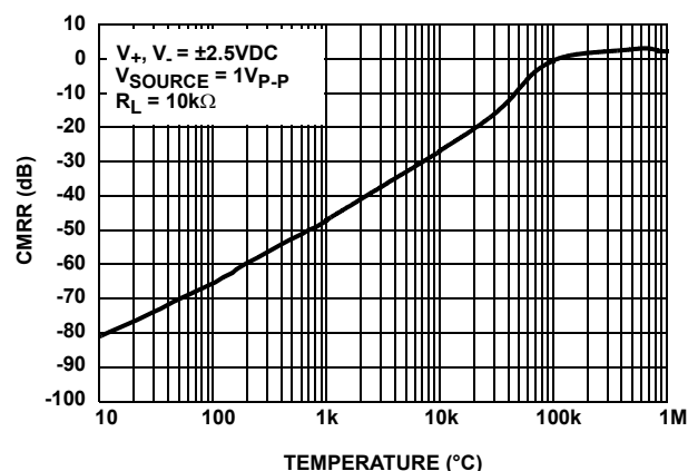
FIGURE 18. AMPLIFIER "B" (OP AMP) CMRR vs FREQUENCY
