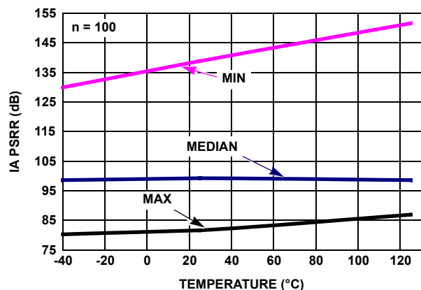
FIGURE 51. IA PSRR vs TEMPERATURE, V_+ = +2.5V , V_- = -2.5V
