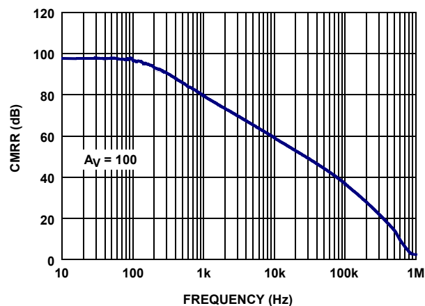
FIGURE 6. AMPLIFIER "A" (IN-AMP) CMRR vs FREQUENCY
