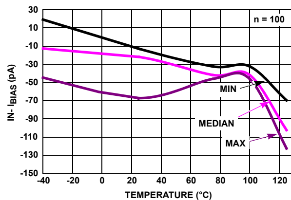
FIGURE 38. I_{BIAS} (IN-) vs TEMPERATURE, V_+ , V_- = \pm 2.5V
