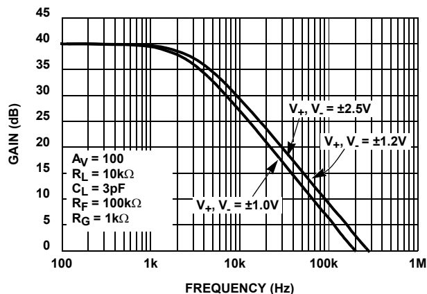
FIGURE 12. AMPLIFIER "B" (OP-AMP) FREQUENCY RESPONSE vs SUPPLY VOLTAGE
