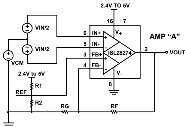
FIGURE 62. GAIN SETTING AND REFERENCE CONNECTION
