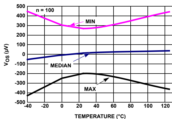
FIGURE 48. INPUT OFFSET VOLTAGE vs TEMPERATURE, V_+, V_- = \pm 1.2V
