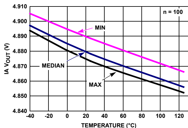
FIGURE 53. IA V_{OUT} HIGH vs TEMPERATURE, R_L = 1k , V_+ = +2.5V , V_- = -2.5V
