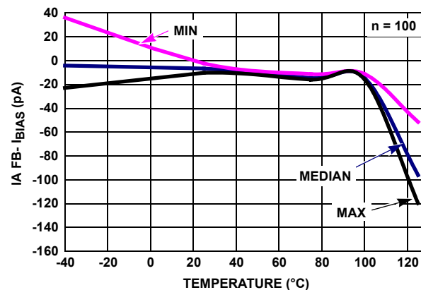
FIGURE 30. I_{BIAS} ( I_{A FB-} ) vs TEMPERATURE, V_+ , V_- = \pm 2.5V
