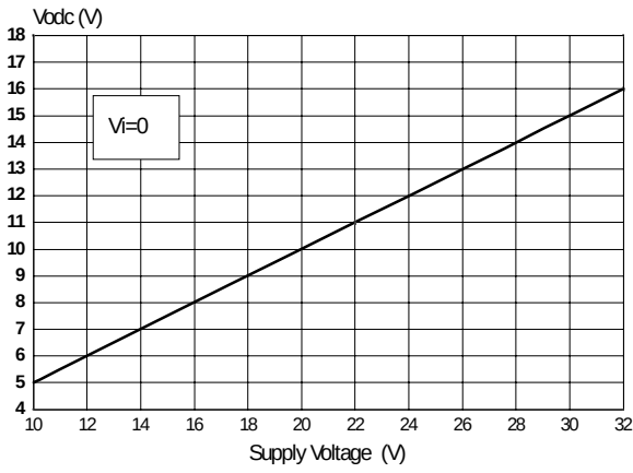
Output DC Voltage vs. Supply Voltage
