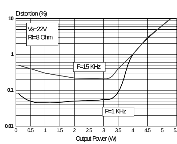
Distortion vs. Output Power
