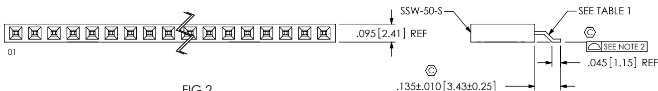
FIG 2 SMH-120-XX-XX-S SHOWN (SAME AS FIG 1, UNLESS OTHERWISE STATED)
