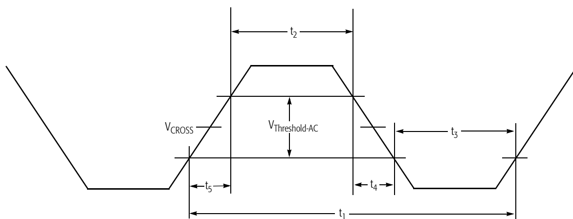
Figure 10. SYSCLK Waveform
