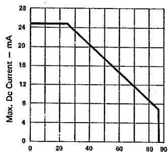
Fig. 4 MAX. ALLOWABLE DC CURRENT PER SEG. Vs AMBIENT TEMPERATURE. Fig. 5 MAX. PEAK CURRENT Vs. DUTY CYCLE.% (REFRESH RATE - F = 1\text{ KHz} ) Fig. 6 LUMINOUS INTENSITY Vs. DUTY CYCLE% (AVERAGE I_F = 10\text{ mA} PER SEG.)
