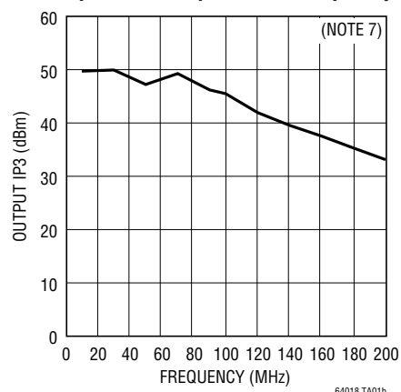
Equivalent Output IP3 vs Frequency
