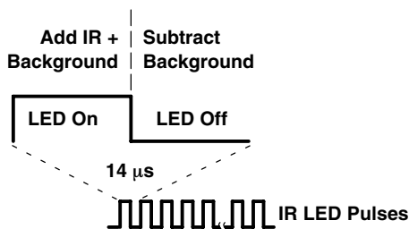
Figure 11. Proximity IR LED Waveform
