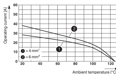
Derating diagram
