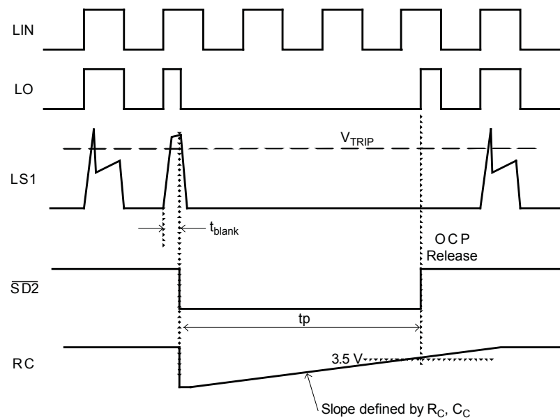
OCP Timing Diagram
