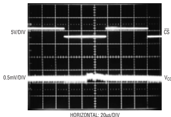
Figure 6. Lithium Battery with 10\mu\text{F} Bypassing on V_{CC}
