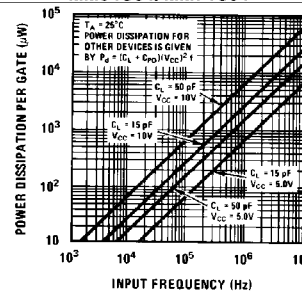
Power Dissipation vs Frequency MM54C00/MM74C00, MM54C02/MM74C02, MM54C04/MM74C04
