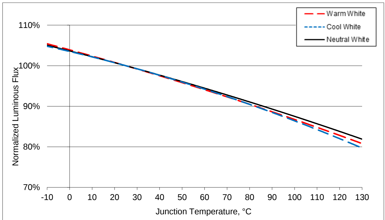
Figure 3: Typical Flux vs. Junction Temperature
