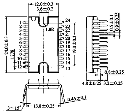
24-pin Shrink DIL Plastic Package (SDIP024-P-0550)
