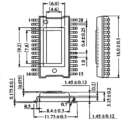
28-pin PANAFLAT Plastic Package (HSOP028-P-0450)
