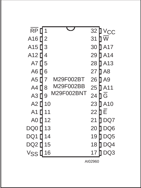
Figure 2C. PDIP Connections
