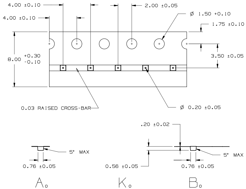
Figure 51. Flip-chip 4 tape
