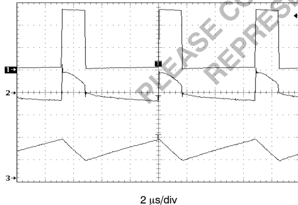
Figure 41. NCP1402SN30T1 Operating Waveforms (Medium Load)
