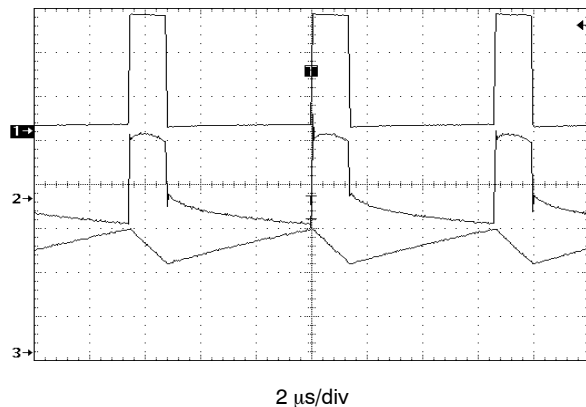
Figure 42. NCP1402SN30T1 Operating Waveforms (Heavy Load)
