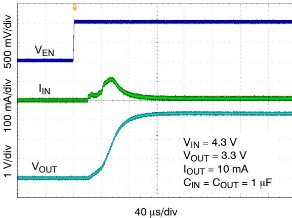
Figure 32. Enable Turn-on Response – V OUT = 3.3 V, C OUT = 1 \mu F
