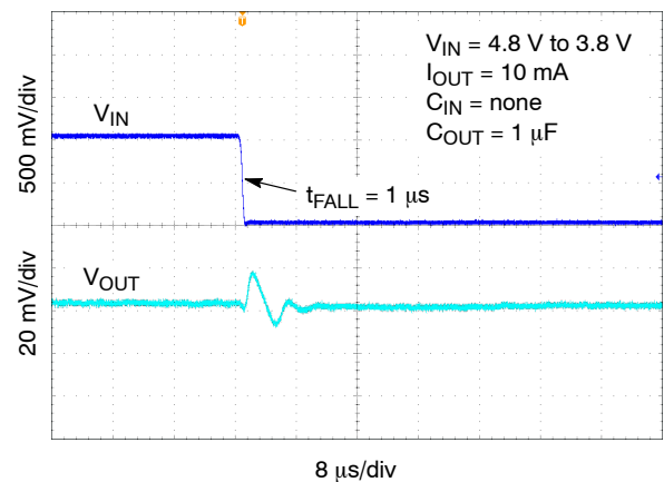
Figure 35. Line Transient Response – Falling Edge, V OUT = 3.3 V, I OUT = 10 mA
