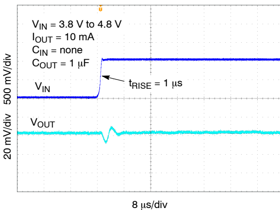
Figure 34. Line Transient Response – Rising Edge, V OUT = 3.3 V, I OUT = 10 mA
