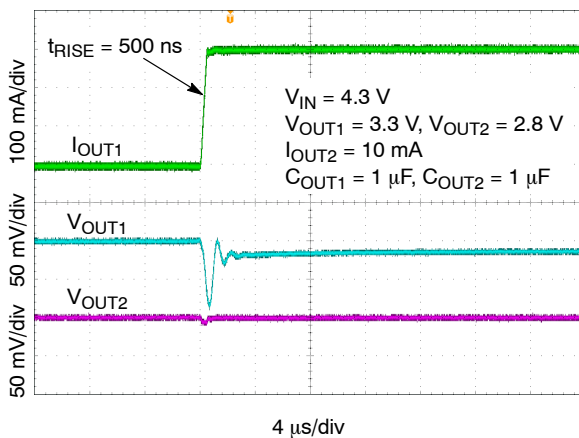
Figure 46. Load Transient Response – 3.3 V – Rising Edge, I_{OUT1} = 100\text{ }\mu\text{A} to 300 mA
