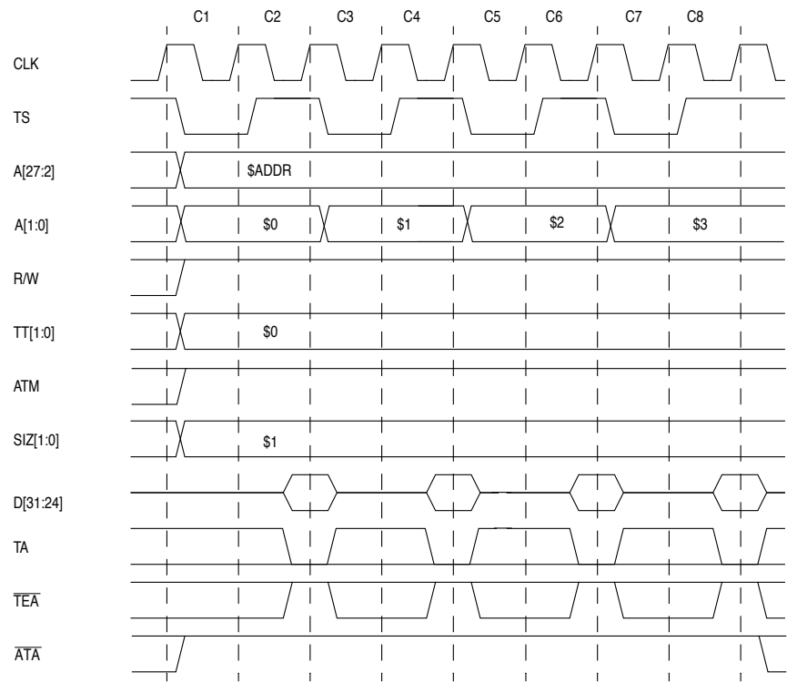
Figure 6-13 shows a burst-inhibited supervisor code longword-read transfer from an 8-bit port.
