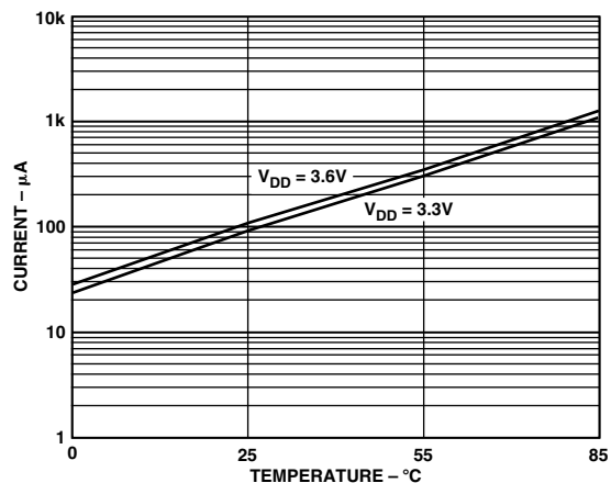
Figure 29. Power-Down Graph
